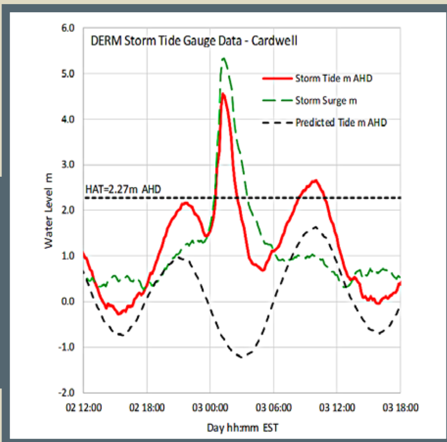
Reconstructed Yasi storm tide event based on the Cardwell tide gauge
