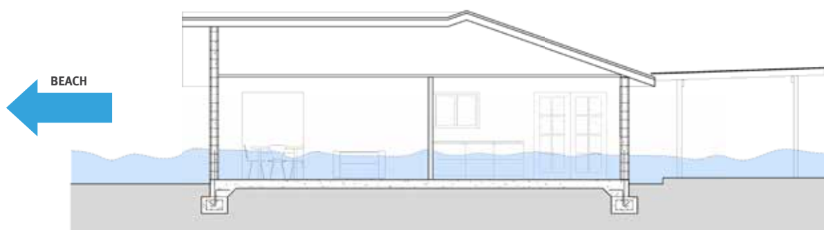
Single storey flow through design for Exposure W homes
