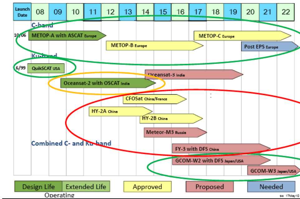
Fig 13. The planned constellation of OVW satellite missions. The colors of the bars indicate whether the mission has been launched, approved, proposed or needed. The circles indicate timeliness of the data; Green indicate data is available in time for operational uses, yellow circles indicate that efforts are underway to make these available in a timely manner, and red circles indicate that timeliness issues have yet been determined. (S. Wilson, personal communication)
